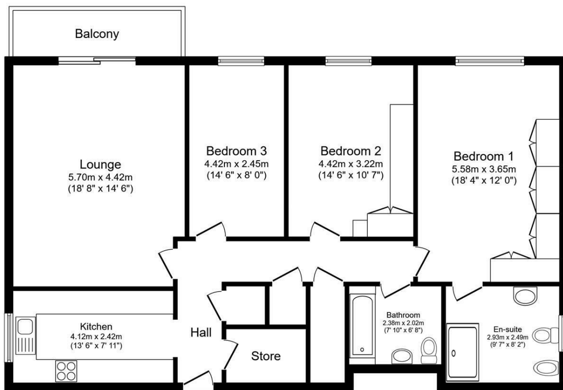
Floor Plan
