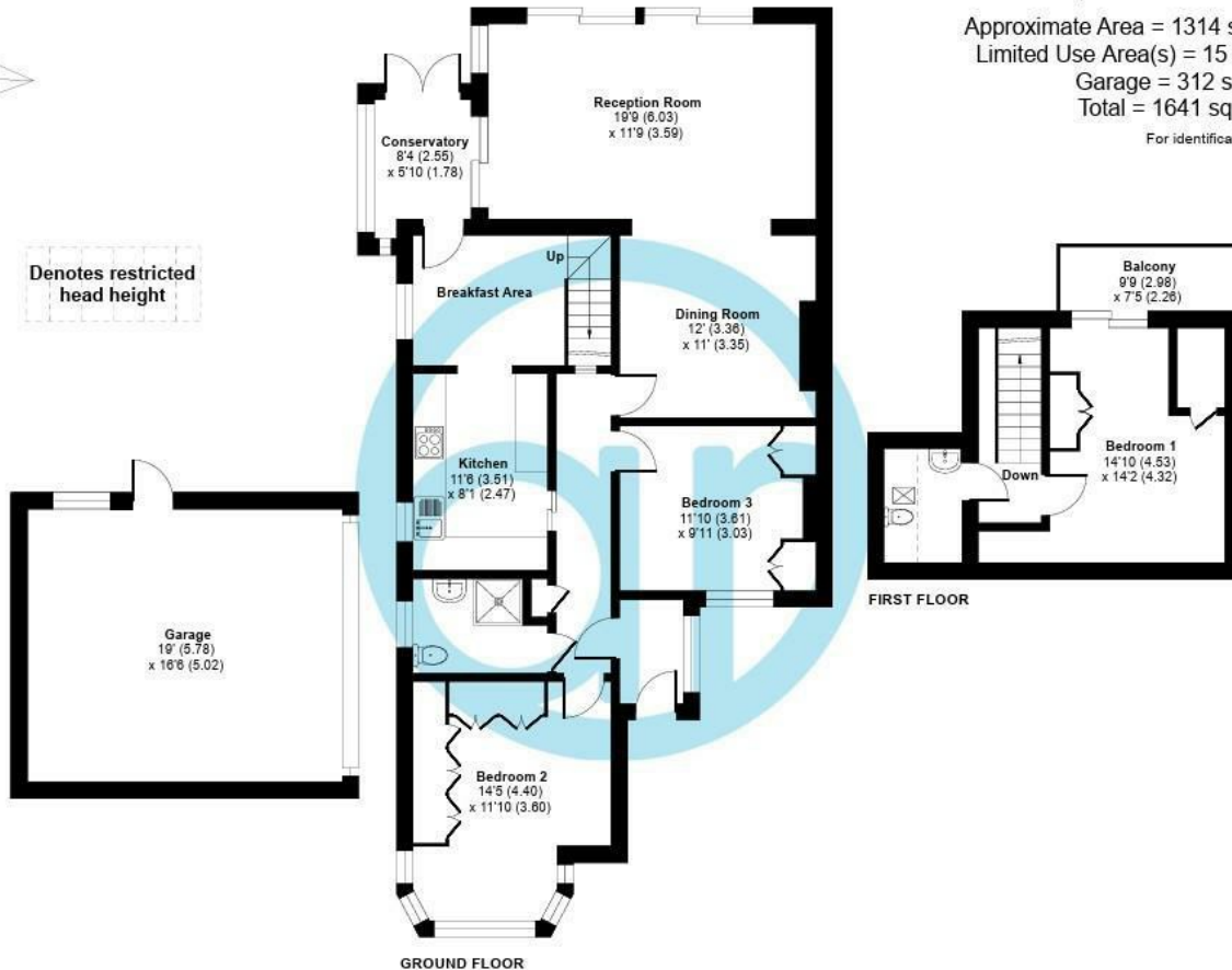
GROUND FLOOR
